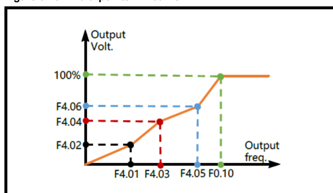
Figure 6-10 Multi-points V/F curve
