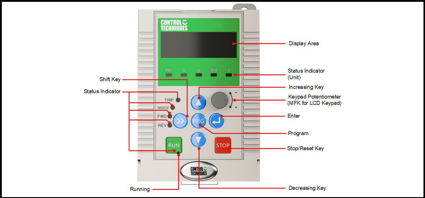
Figure 5-1 Keypad diagram
