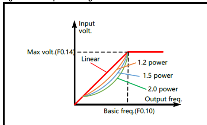
Figure 6-9 Torque-reducing curve
