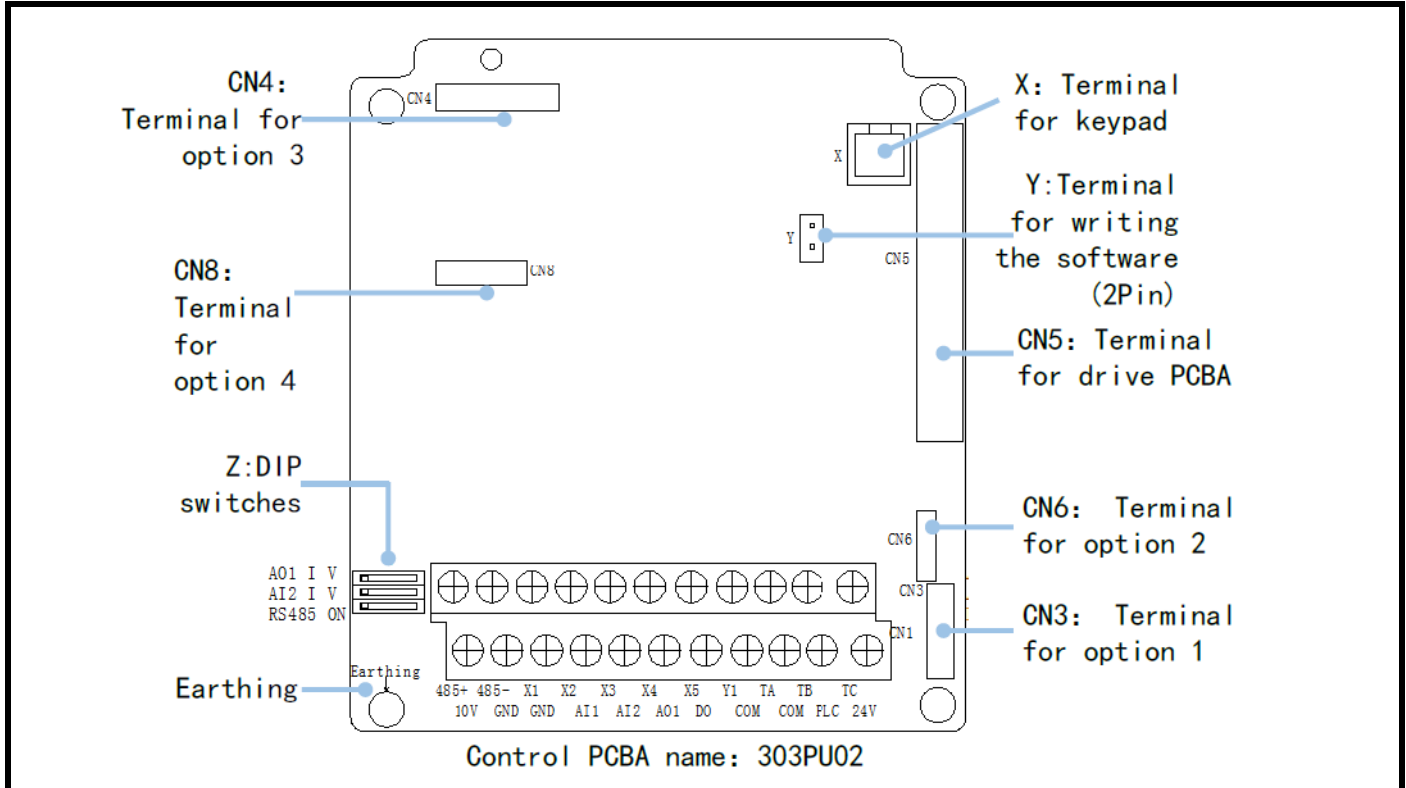
Figure 4-28 NE300 close-loop control PCBA diagram
