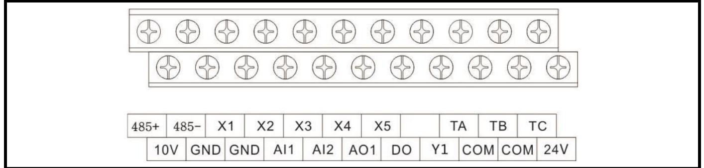
Figure 4-17 Control circuit terminals diagram
