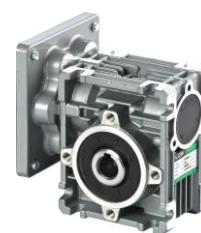
Worm Gearhead (Right Angle - Hollow) Single Gear Reduction Ratio 1/5 to 1/80 (1/100)
